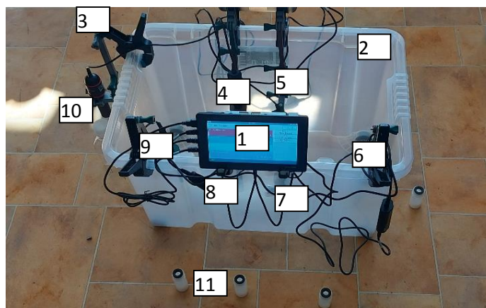
Fig. 1. General view of the mobile measurement system
